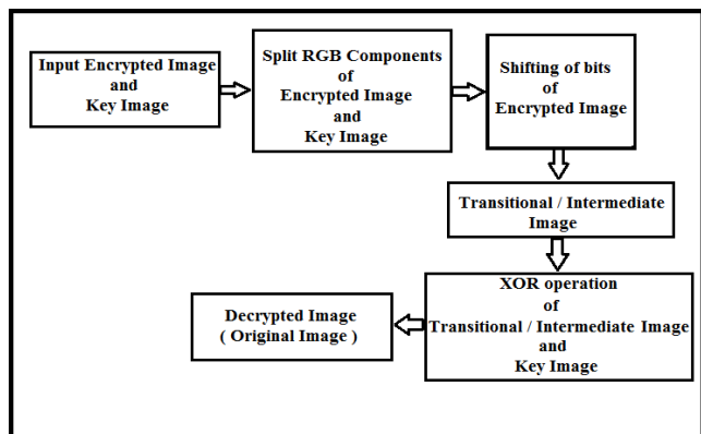
Fig.9 RGB pixel displacement Decryption
