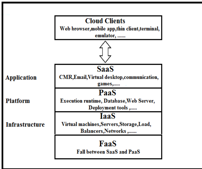
Fig.2 Service model
