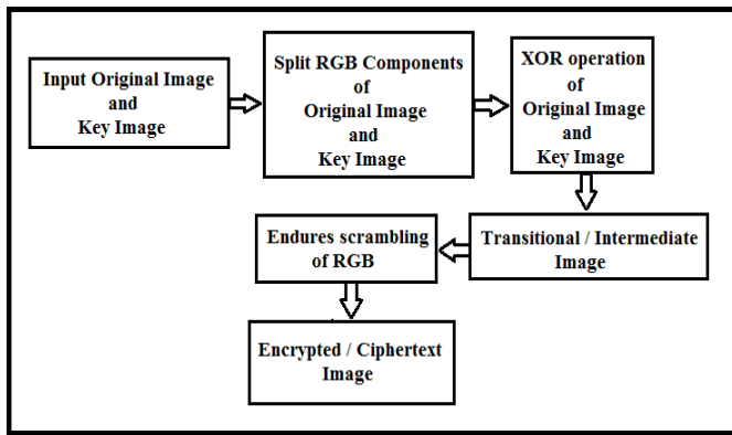
Fig.5 RGB pixel displacement Encryption
