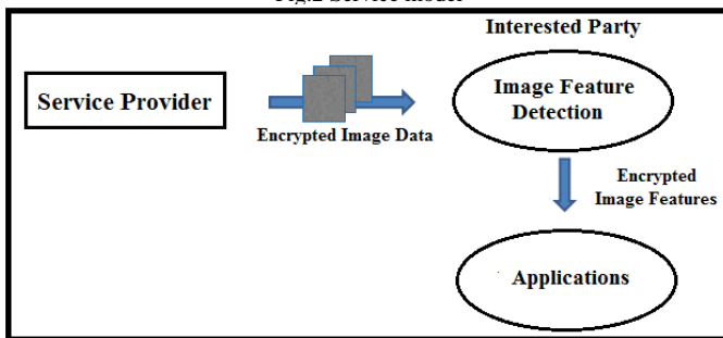
Fig.3 Cloud System Model
