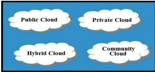
Fig.1 Deployment Model
