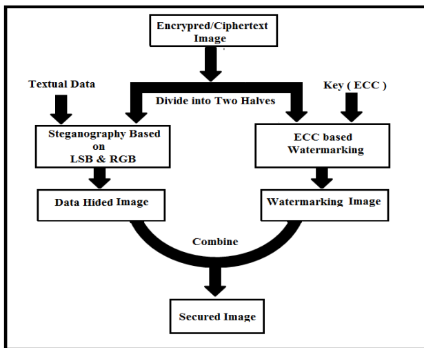
Fig.7 Framework in Cloud
